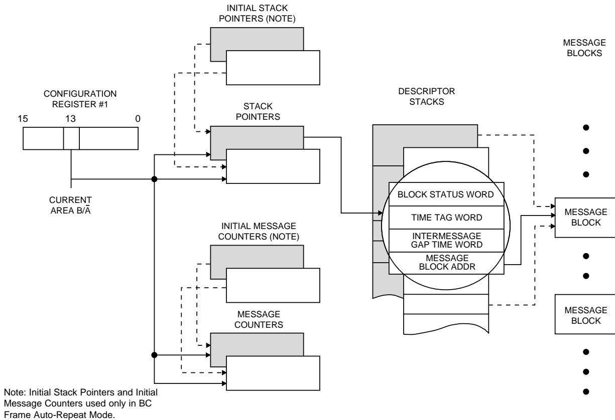
FIGURE 8. BC MODE MEMORY MANAGEMENT
